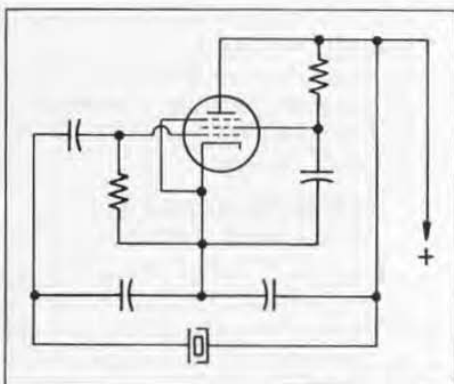
Figure 2. Elementary schematic circuit of the crystal oscillator. The crystal operates only slightly off resonance, at a frequency where its inductive reactance is equal to the reactance of the two capacitors.
