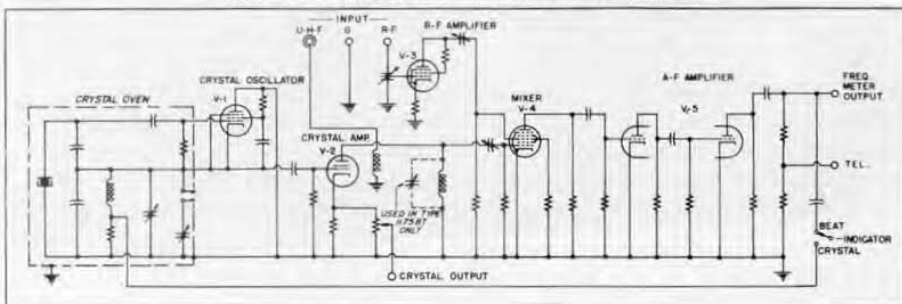
Figure 3. Elementary schematic circuit of the complete monitor.
